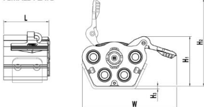
FEMALE PLATE
